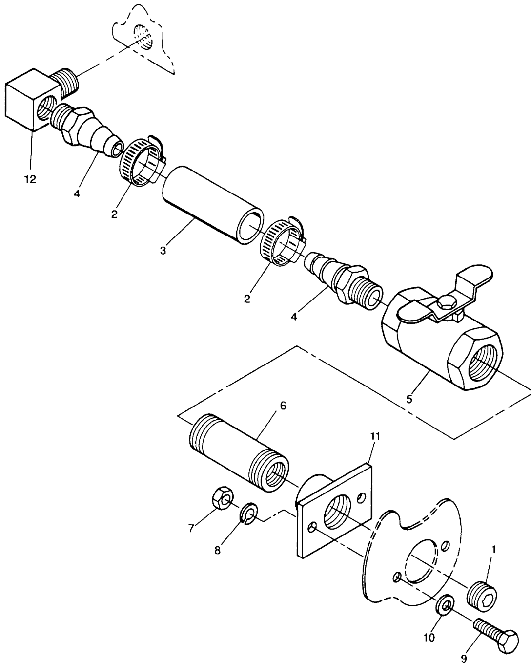
Figure 18. Oil Drain Line
