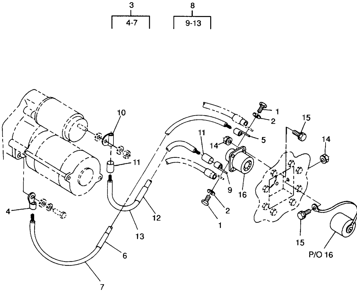
Figure 2. Slave Receptacle and Cables
